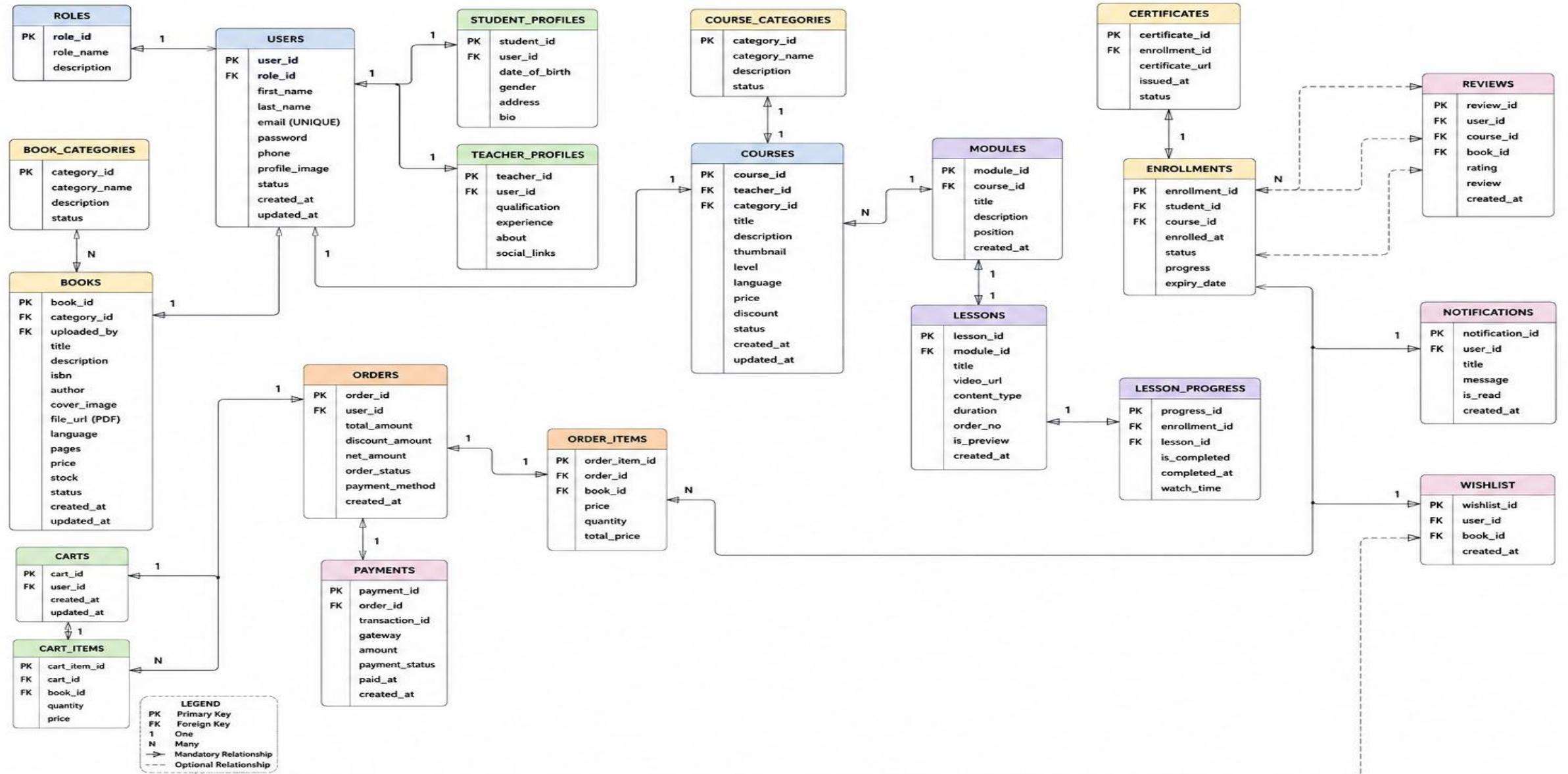
ER DIAGRAM – EDUVERSE (E-Book Store + E-Learning Platform)
